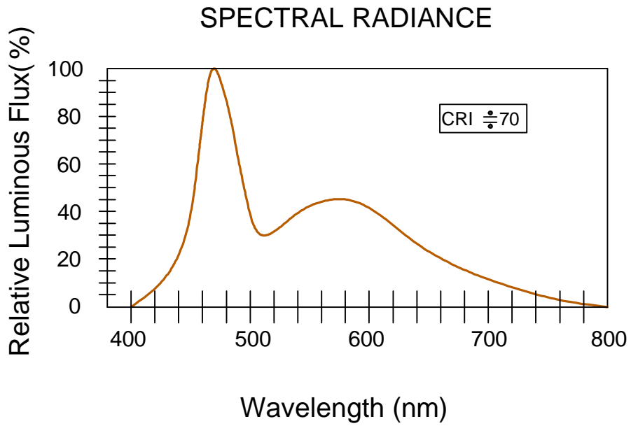
Fig.5 Luminous Spectrum(Ta=25 )
